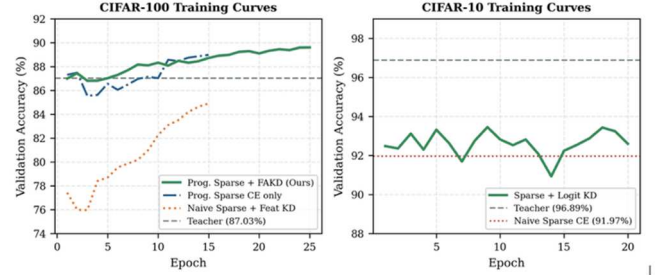
Fig. 4. Validation accuracy during training. Left: CIFAR-100—PTP-FAKD crosses teacher baseline (87.03%) at epoch 7 and converges to 89.60%. Right: CIFAR-10—logit KD recovers 1.48% over naive sparse CE baseline.
