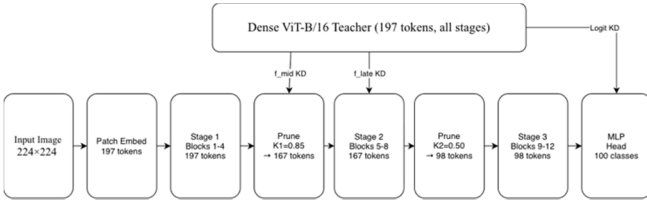
Fig. 1. PTP-FAKD architecture. Tokens are pruned progressively after Stage 1 ( \kappa_1=0.85 , 197 \rightarrow 167 tokens) and Stage 2 ( \kappa_2=0.50 , 167 \rightarrow 98 tokens). FAKD aligns intermediate L_2 -normalized CLS representations \hat{\mathbf{f}}_{\text{late}}^s and \hat{\mathbf{f}}_{\text{mid}}^t , and output logit distributions, with the frozen dense teacher.
