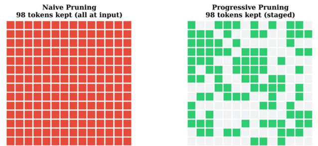
Fig. 5. Token retention visualization at 50% budget. Naive pruning (left) selects high-norm embedding-level tokens regardless of spatial coherence. Progressive pruning (right) retains semantically concentrated, spatially coherent tokens after two rounds of post-processing selection, supporting the implicit regularization hypothesis.
